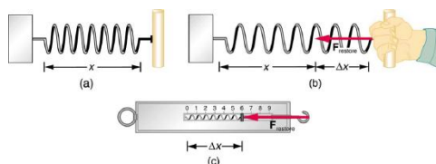
Figure 2.2.1: The force exerted by a stretched spring can be used as a standard unit of force. (a) This spring has a length x when undistorted. (b) When stretched a distance \Delta x , the spring exerts a restoring force, \mathbf{F}_{\text{restore}} , which is reproducible. (c) A spring scale is one device that uses a spring to measure force. The force \mathbf{F}_{\text{restore}} is exerted on whatever is attached to the hook. Here \mathbf{F}_{\text{restore}} has a magnitude of 6 units in the force standard being employed.
